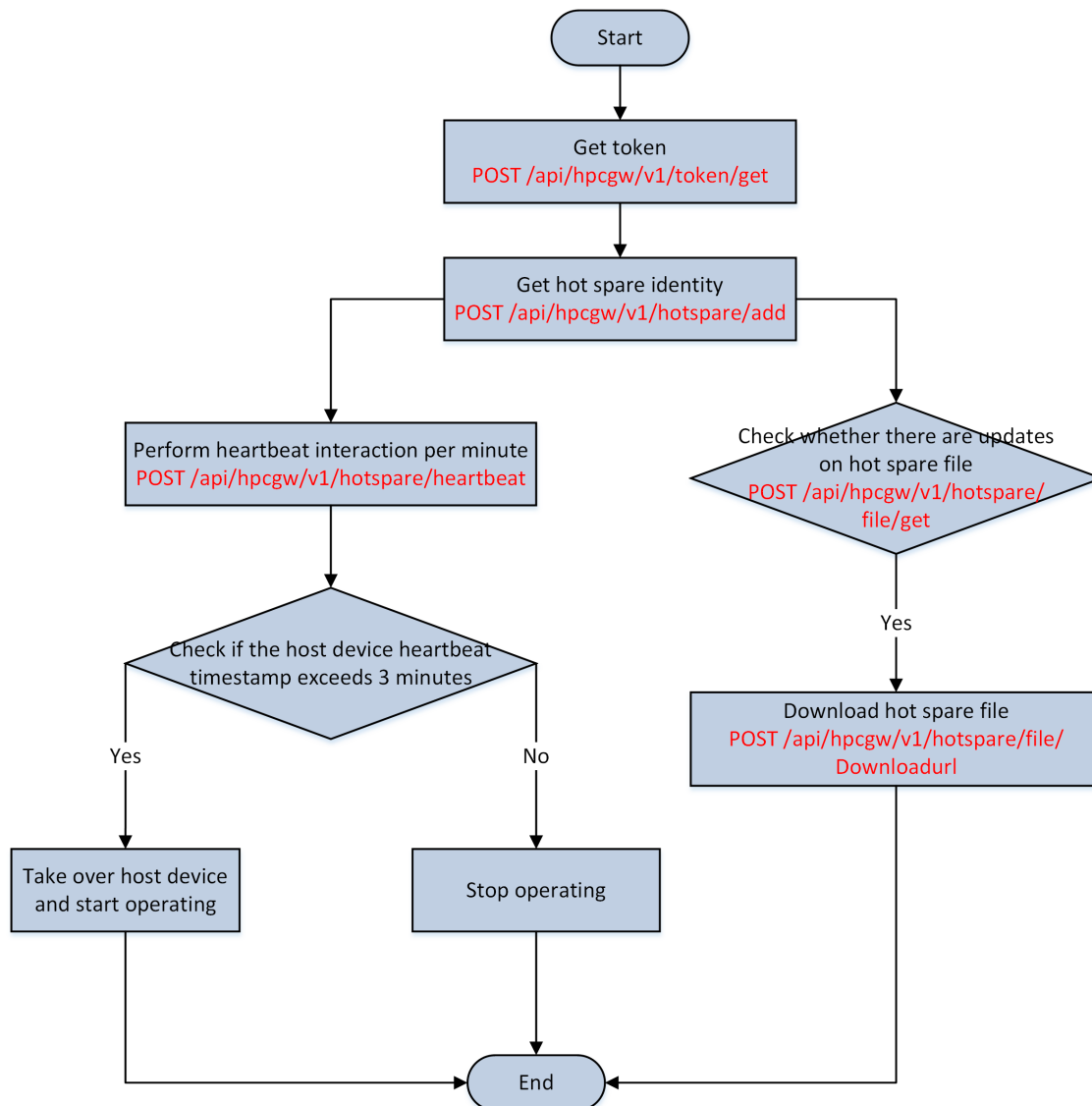
Figure 2-11 API calling flow of Hot Spare (Spare)
