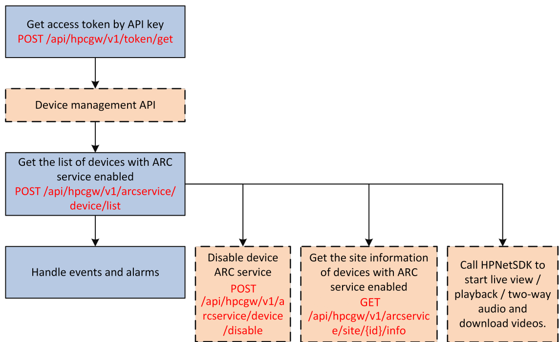
Figure 2-8 ARC Services Integration Flow
