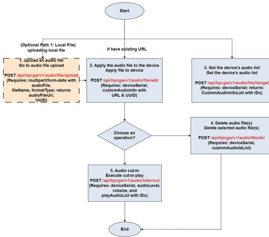
Figure 2-13 API Calling Flow for Audio & Video
